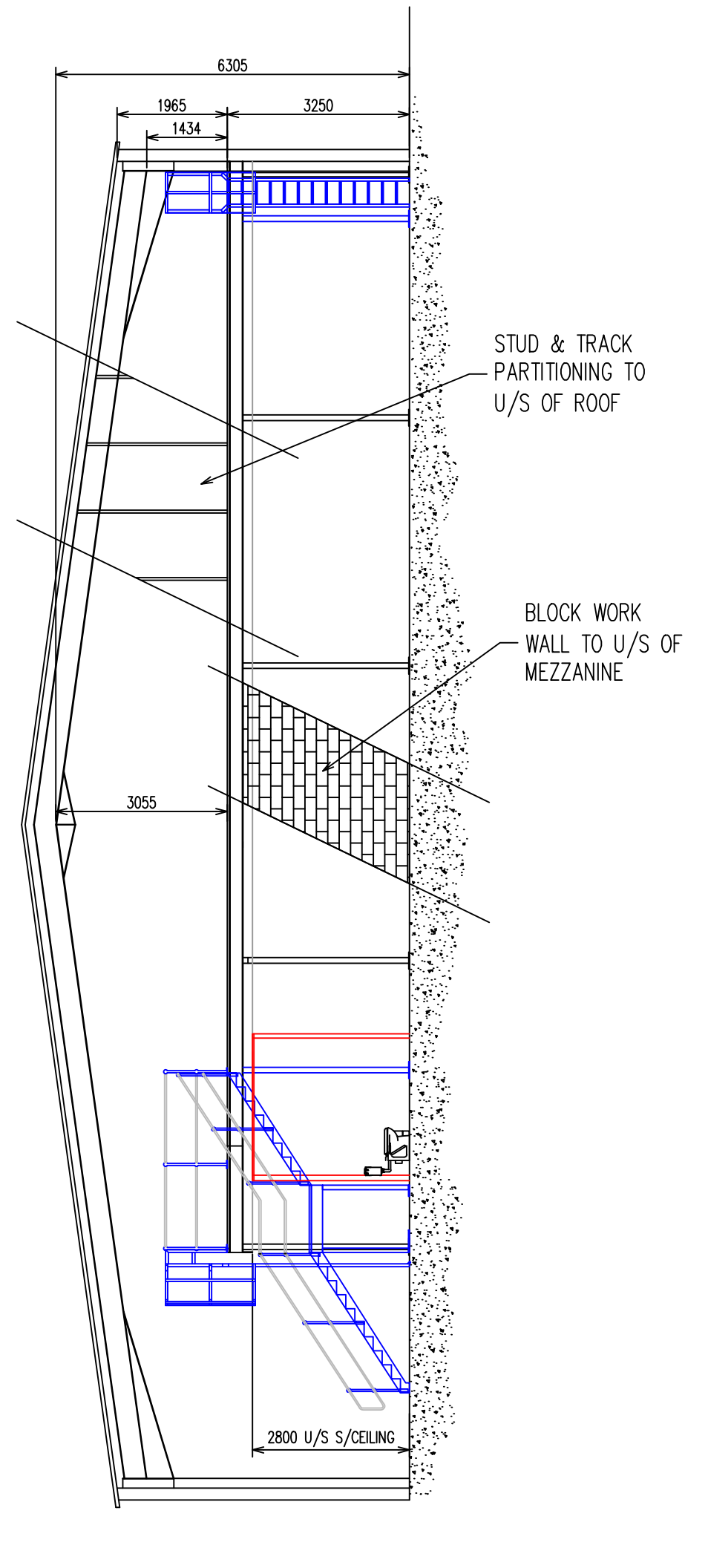
PROPOSED SECTION THROUGH X - X
