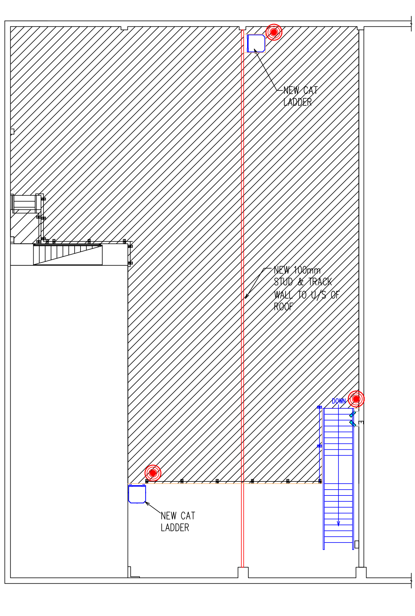
PROPOSED FIRST FLOOR LAYOUT - PLAN VIEW
