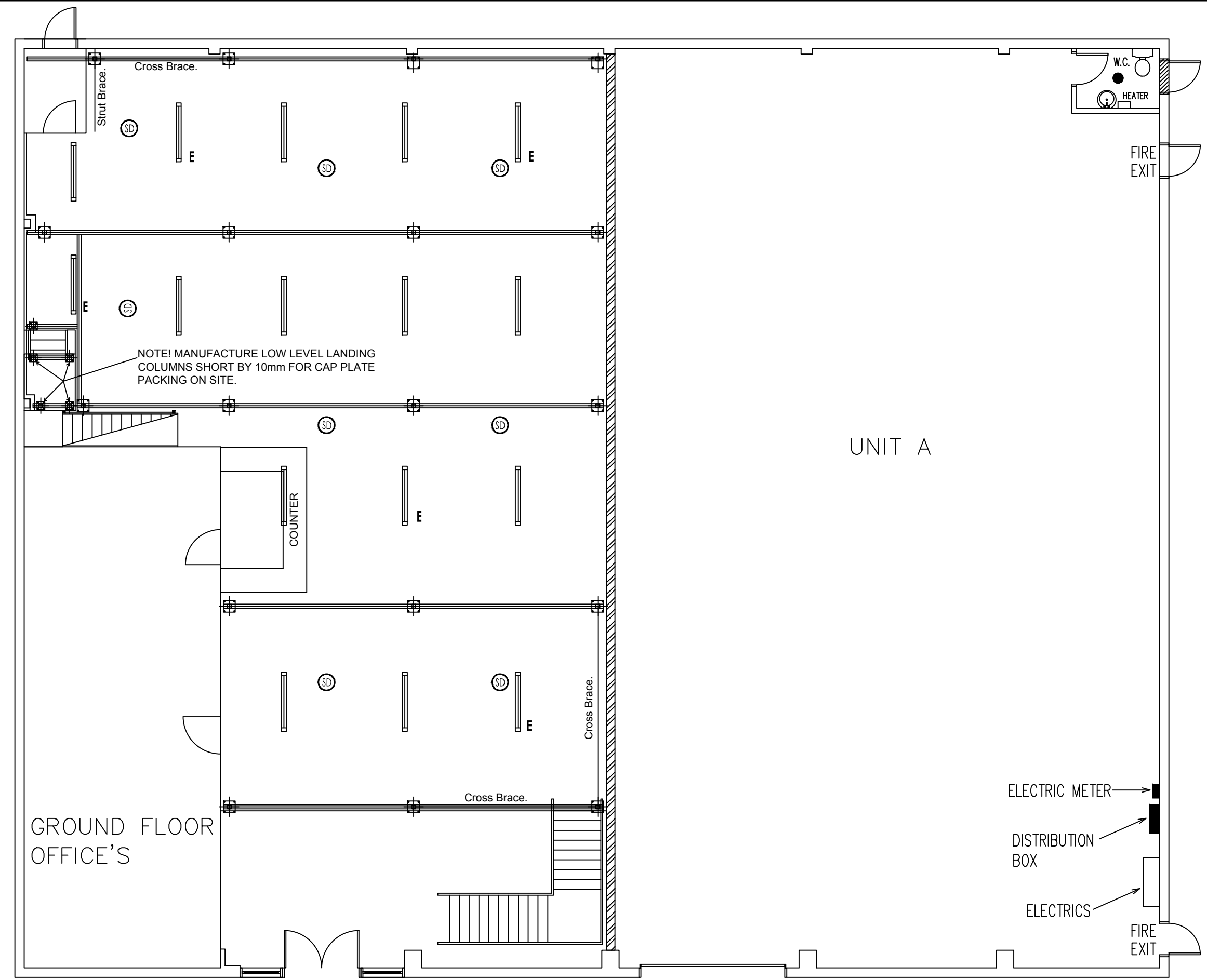
EXISTING GROUND FLOOR LAYOUT - PLAN VIEW
