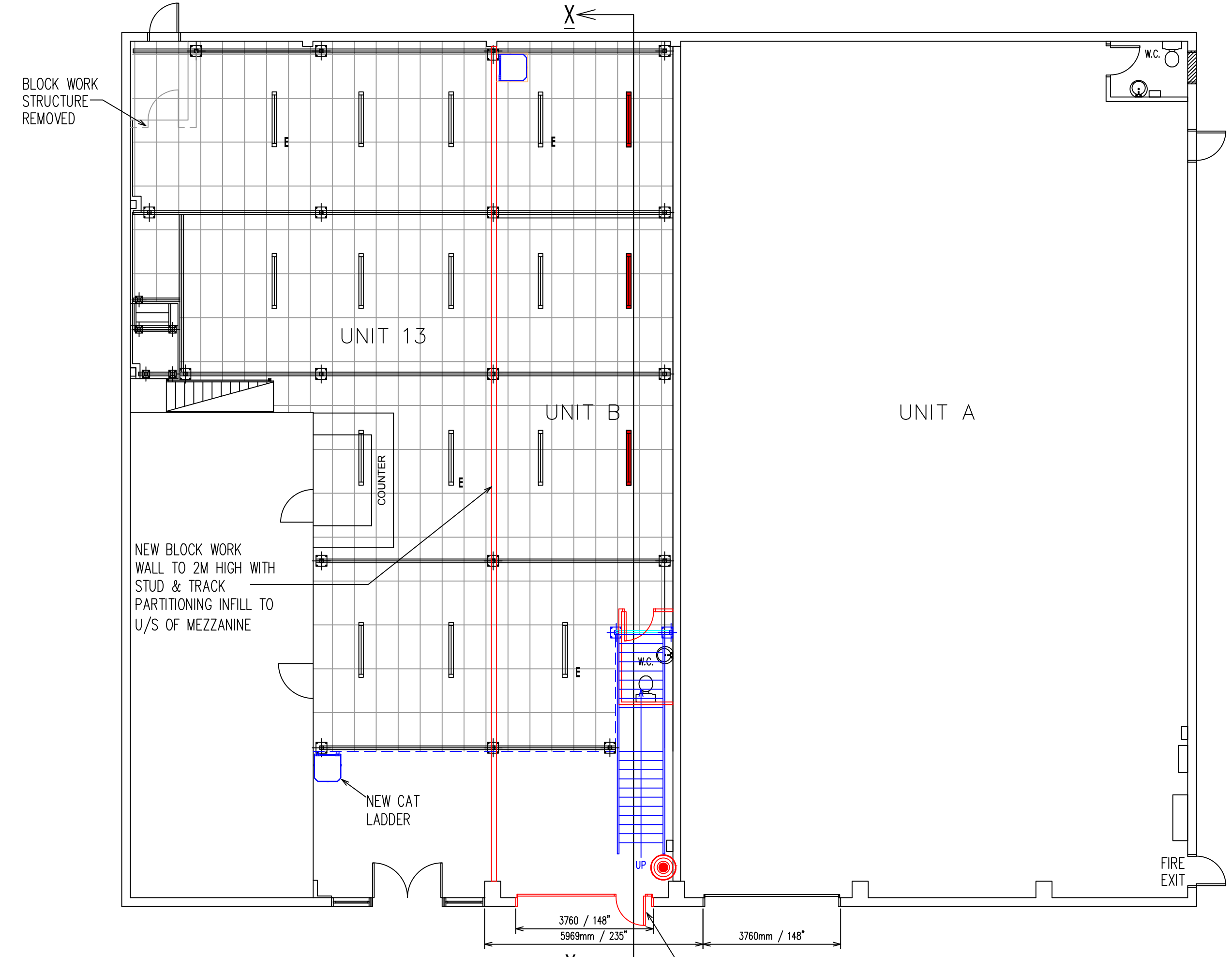
PROPOSED GROUND FLOOR LAYOUT - PLAN VIEW
