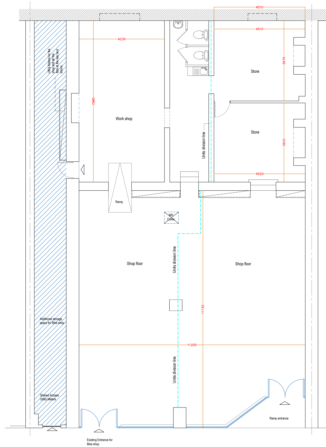
No. 40-42 CLAPHAM HIGH STREET EXISTING FLOOR PLAN
