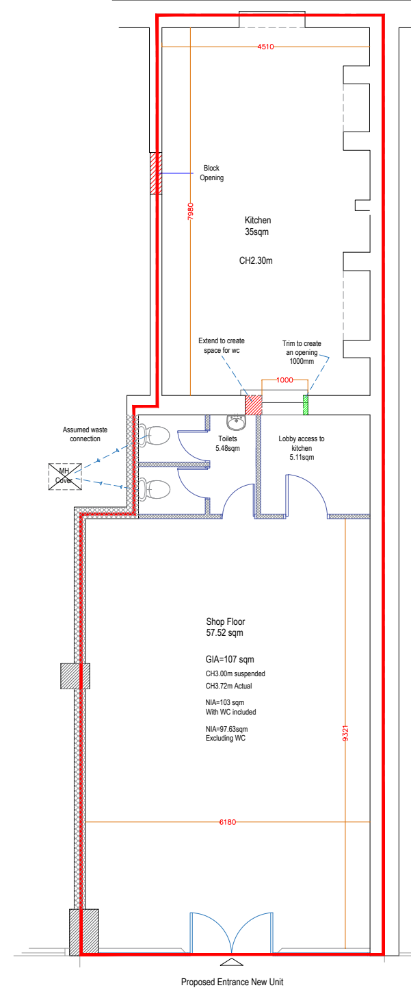
No. 42 CLAPHAM HIGH STREET PROPOSED FLOOR PLAN
