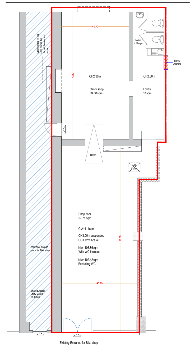
No. 40 CLAPHAM HIGH STREET PROPOSED FLOOR PLAN
